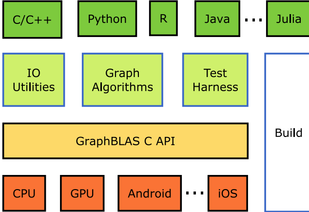
Fig. 1: LAGraph Project Overview. The project consists of a library of graph algorithms and assorted components to support algorithm development and validation (a test harness and I/O utilities). It must interface to a wide range of languages. Underneath these components is a build system, implementations of the GraphBLAS, and a variety of hardware targets.
