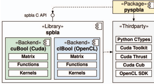
Fig. 1. Sparse Boolean linear algebra library architecture.
